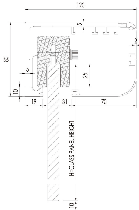
TRACK PROFILE
