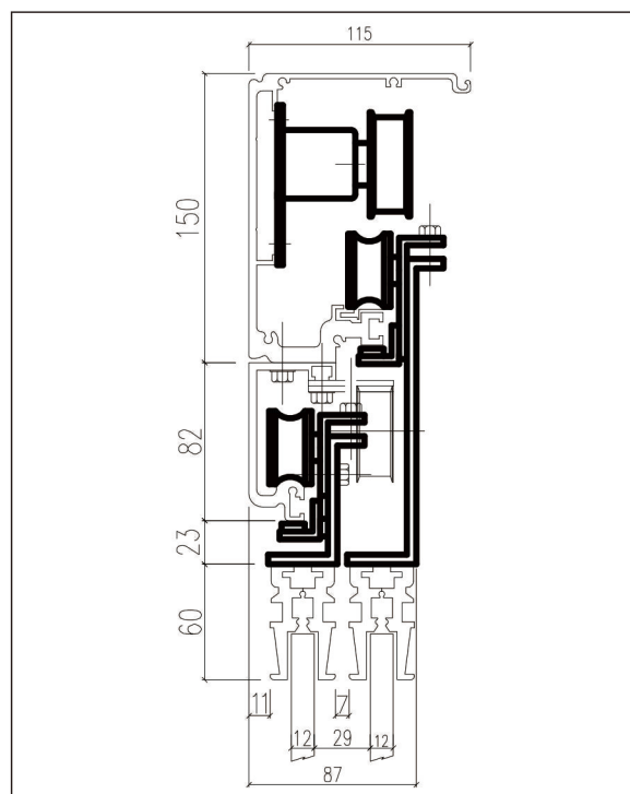
Installation dimensions
